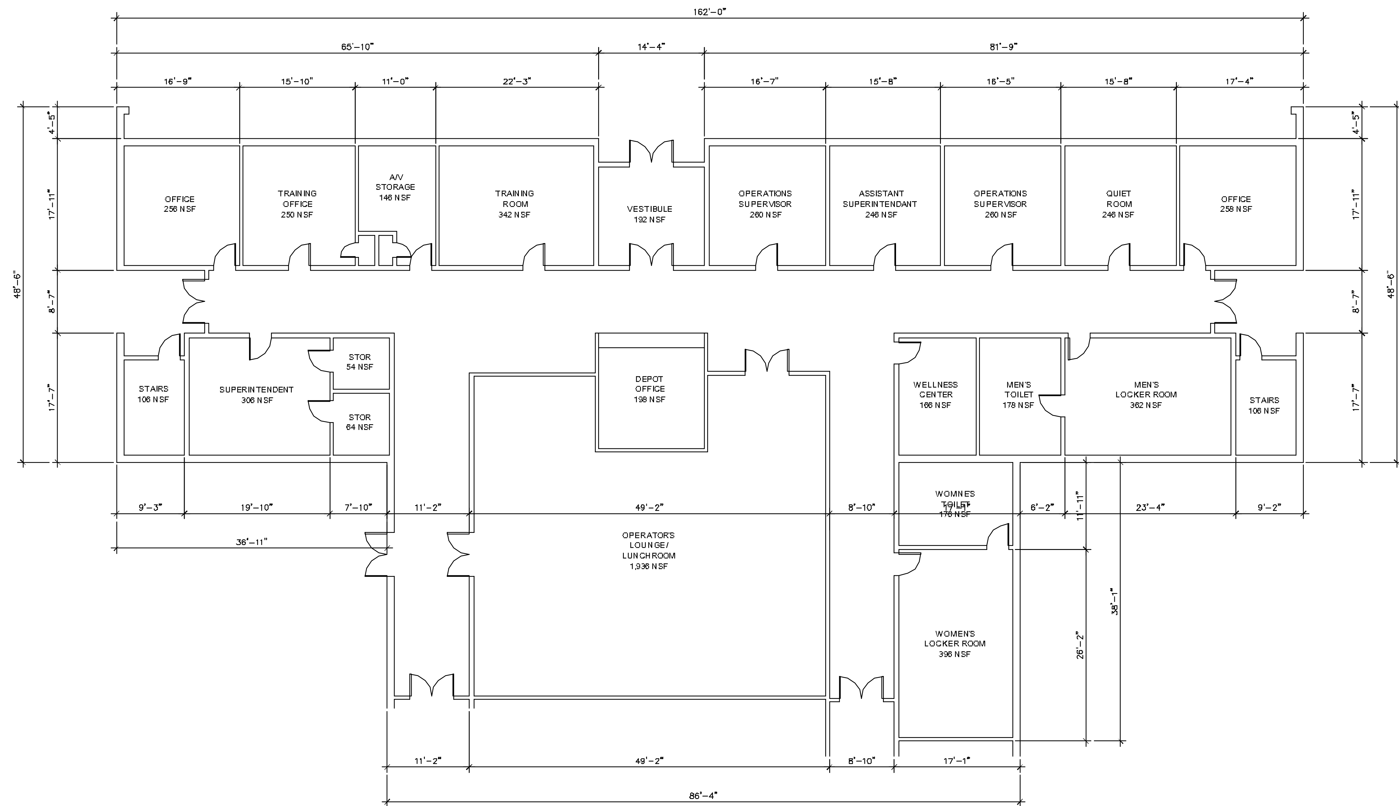
FLOOR PLAN 1/8" = 1'-0"
